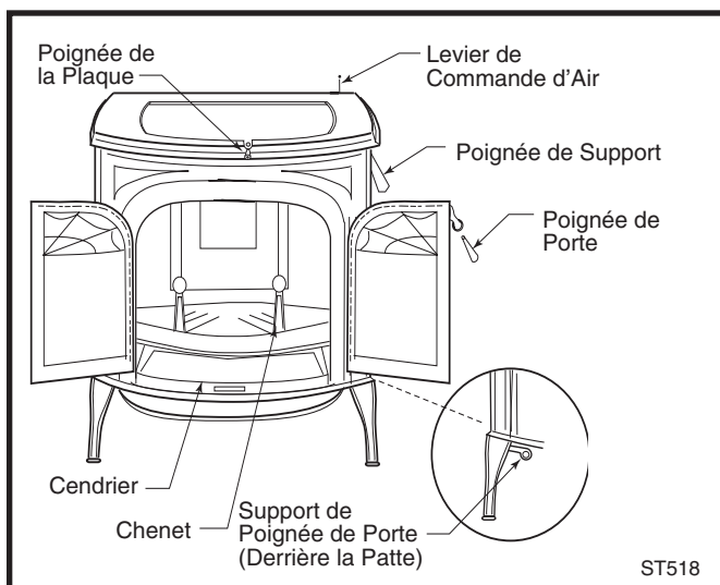
Fig. 32 Commandes poêle Intrepid II.
